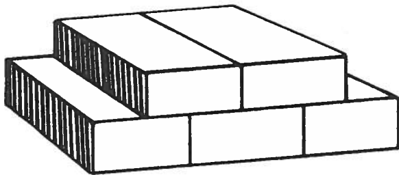
Fig. 2—1: Header course, with bricks laid across the wall.
