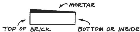
Fig. 2—20: Applying mortar to form a wedge.
