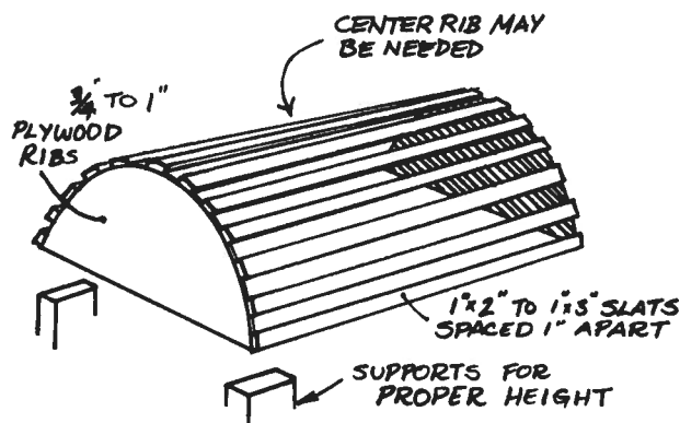
Fig. 2-25: Building a reusable arch form.
