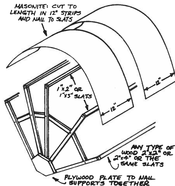
Fig. 2-24: Building a one-use arch form.
