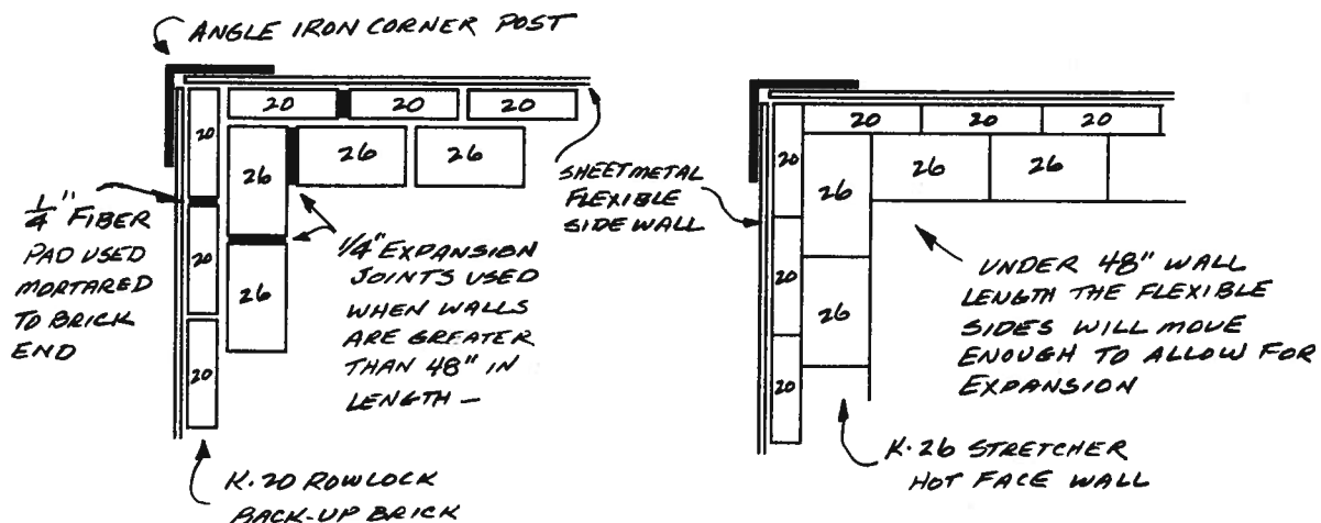
Fig. 2—32: Expansion joint is eliminated in an IFB kiln with steel framework, with a wall 4' or less.
