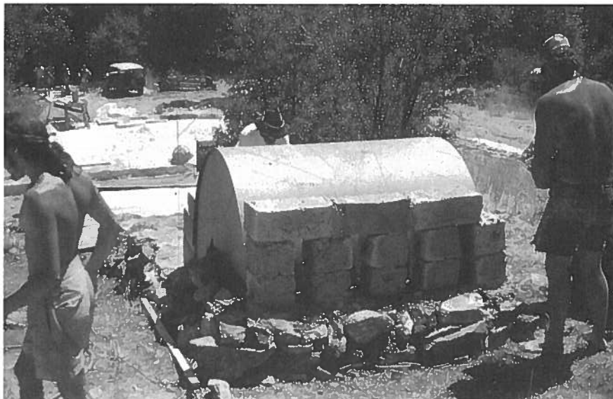
Fig 2—40: Start of straight wall with flue holes.
