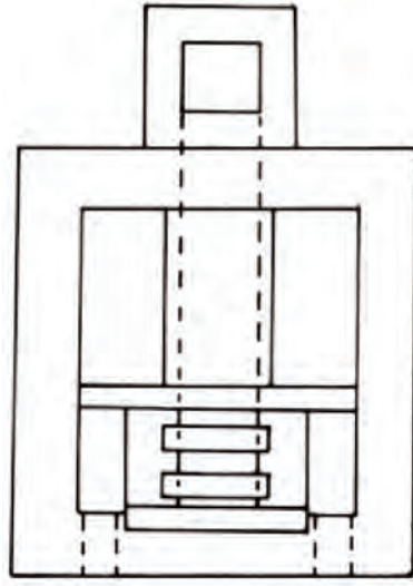
Fig. 4-7. Plan of test kiln. This kiln utilizes the two front burners and soda ports of the downdraft kiln illustrated in Chapter 3. The rear section of the flue channel has been covered with kiln shelves to connect the test kiln to the chimney.
