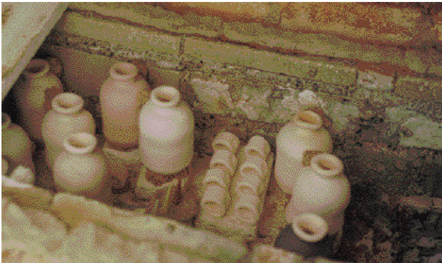
Fig. 4-8. Detail of the pack in the test kiln.
